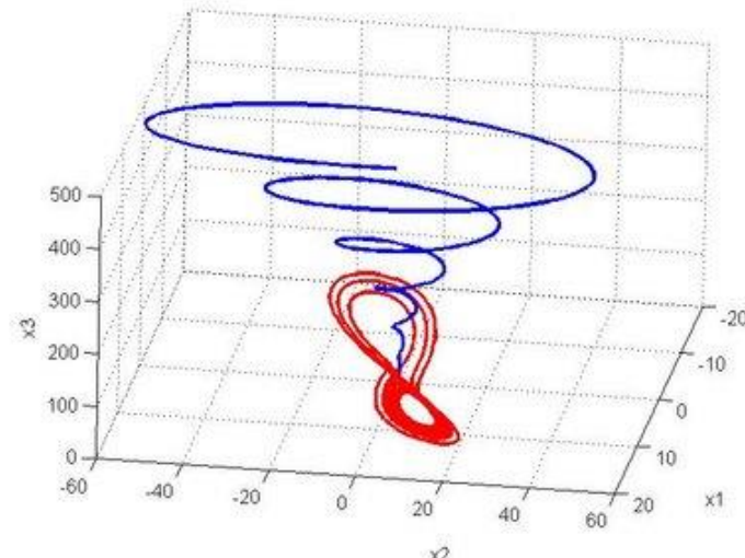
Chaos (Lorenz Attractor)
