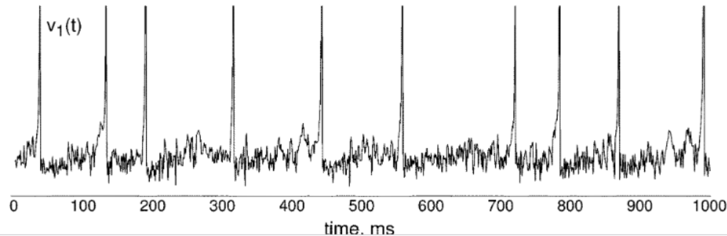
neuron trace
