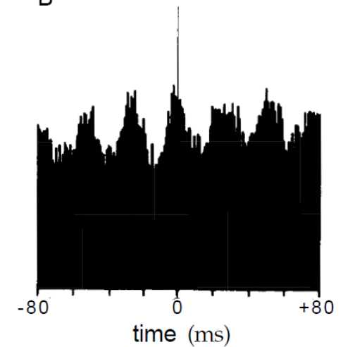
Spike cross-correlations
