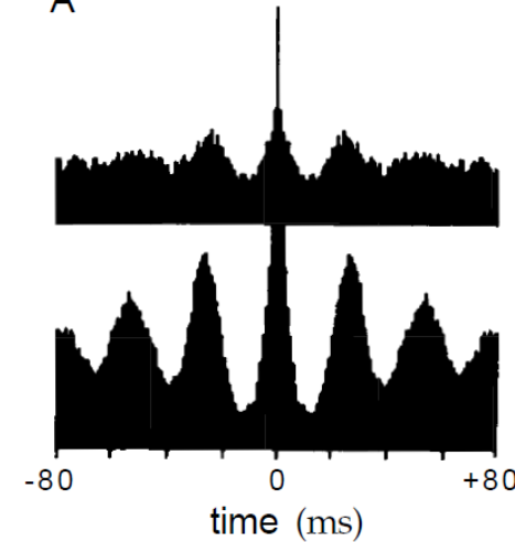
Bursting
