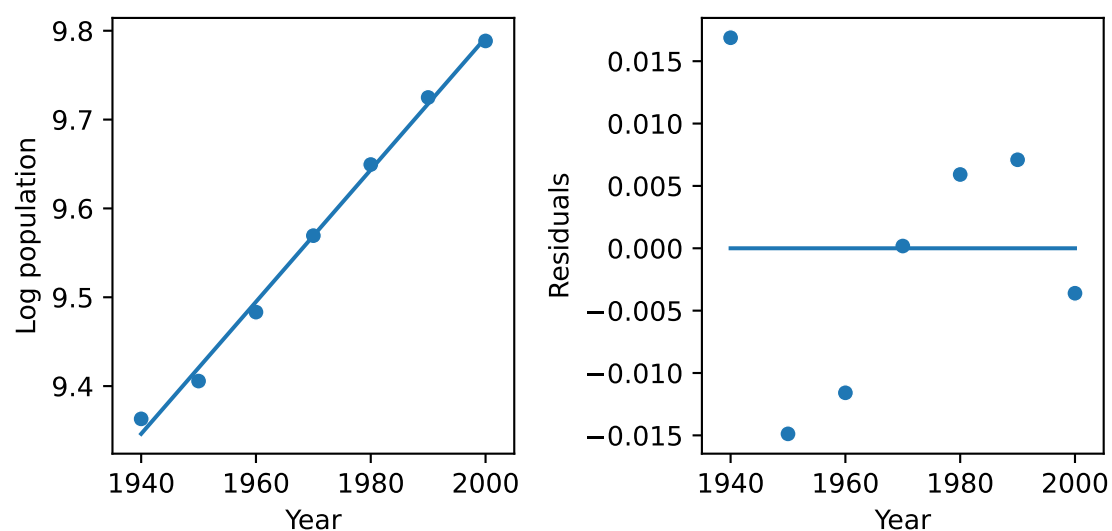
Figure 10.8: Log world population 1940–2000.
