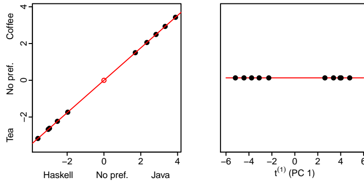
Figure 13.9: Projection into the original space.
