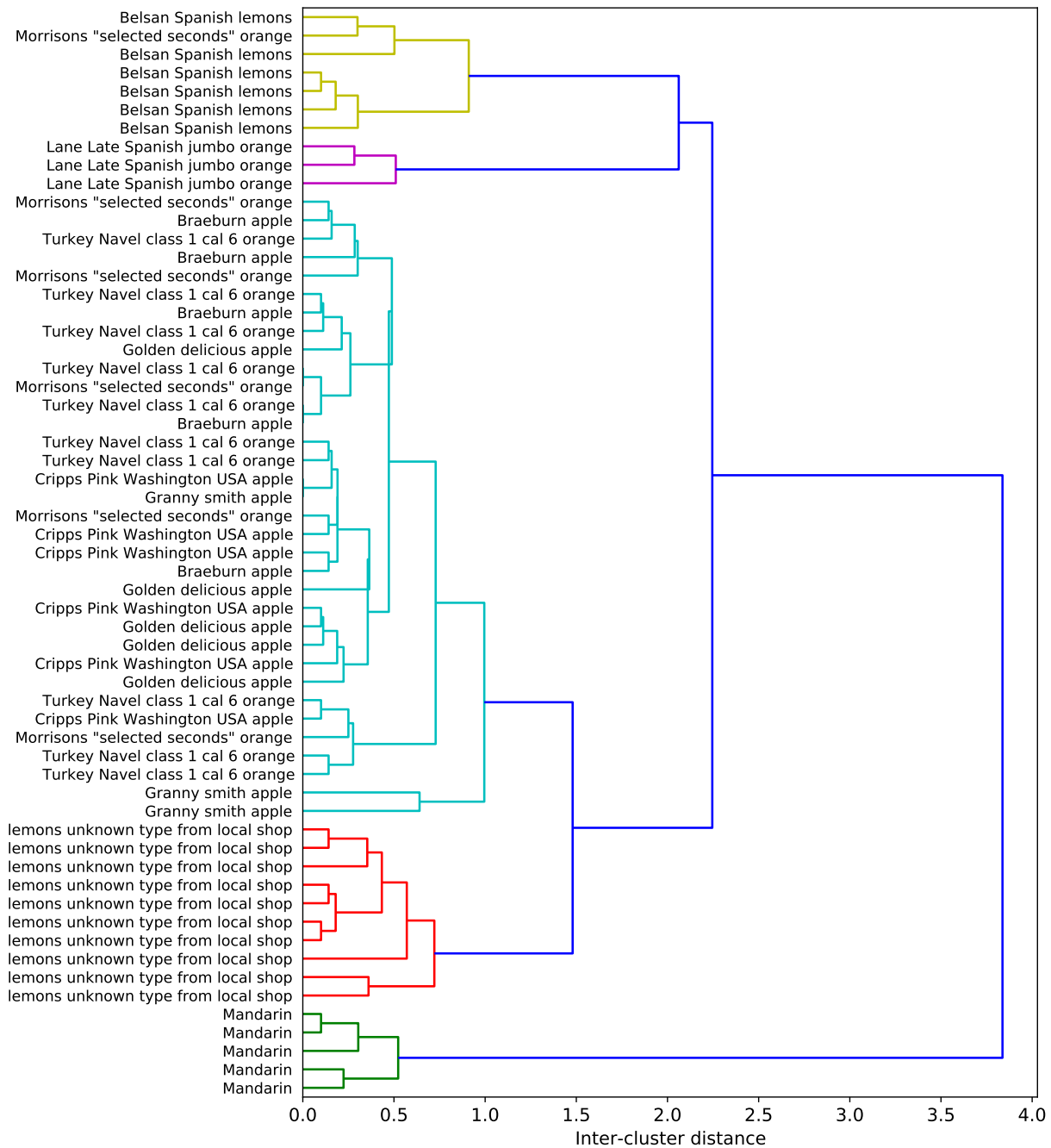
Figure 9.3: Hierarchical clustering of the fruit dataset. The x-axis indicates the distance between clusters, which in this clustering example is the centroid of all the points belonging to the cluster. For example the two Mandarins at the very bottom are about 0.2 units apart, and form a cluster. In turn the centre of this cluster is about 0.45 units from the centre of the next closest cluster (the three other Mandarins). We can regard all sub-trees lower than a threshold inter-cluster distance of our choosing as clusters. For example, if we chose a threshold of 1.0, we would see 5 clusters, indicated by the green, red, cyan, magenta and yellow sub-trees.
