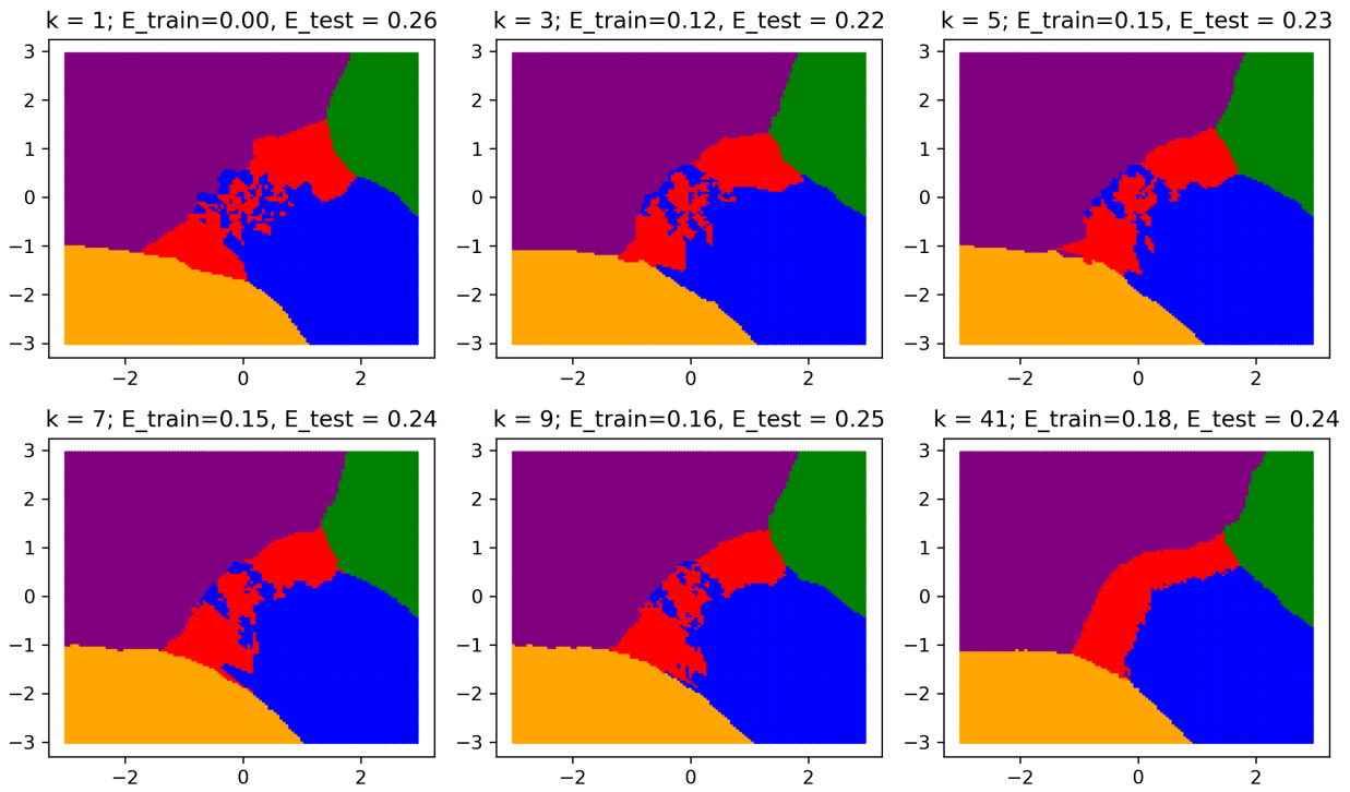
Figure 12.2: Decision regions, training error and testing error for various values of k applied to the 5-fruit data shown in Figure 11.1). Colour indicates decision region for each type of fruit: Apple (blue), Mandarin (orange), Big Orange (green), Orange (red), Lemon (purple).
