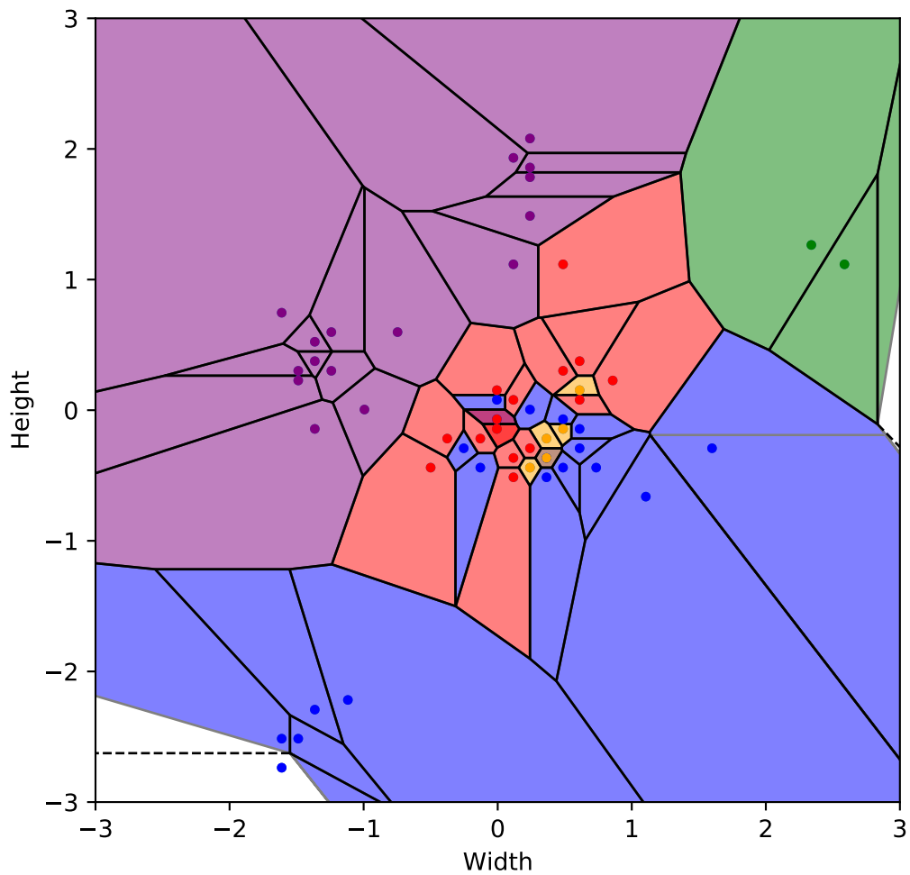
Figure 11.7: Decision regions for one nearest neighbour classification applied to the fruit data set. The variables have been standardised to make the scales on both axes similar. Some regions are darker shade of blue or red. This indicates that there are 2 points labelled with “apple” or “orange” in the dataset with the same features. There is one region that is purple, amongst the blue and red region. There are two data points corresponding to this region with identical coordinates, one labelled with orange and one with apple. Colour indicates decision region for each type of fruit: Apple (blue), Mandarin (orange), Big Orange (green), Orange (red), Lemon (purple).
