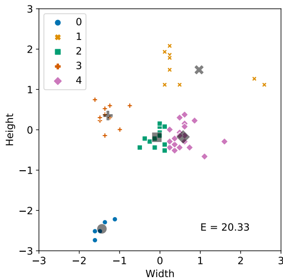
(c) Within-cluster sum-squared error E = 20.33
