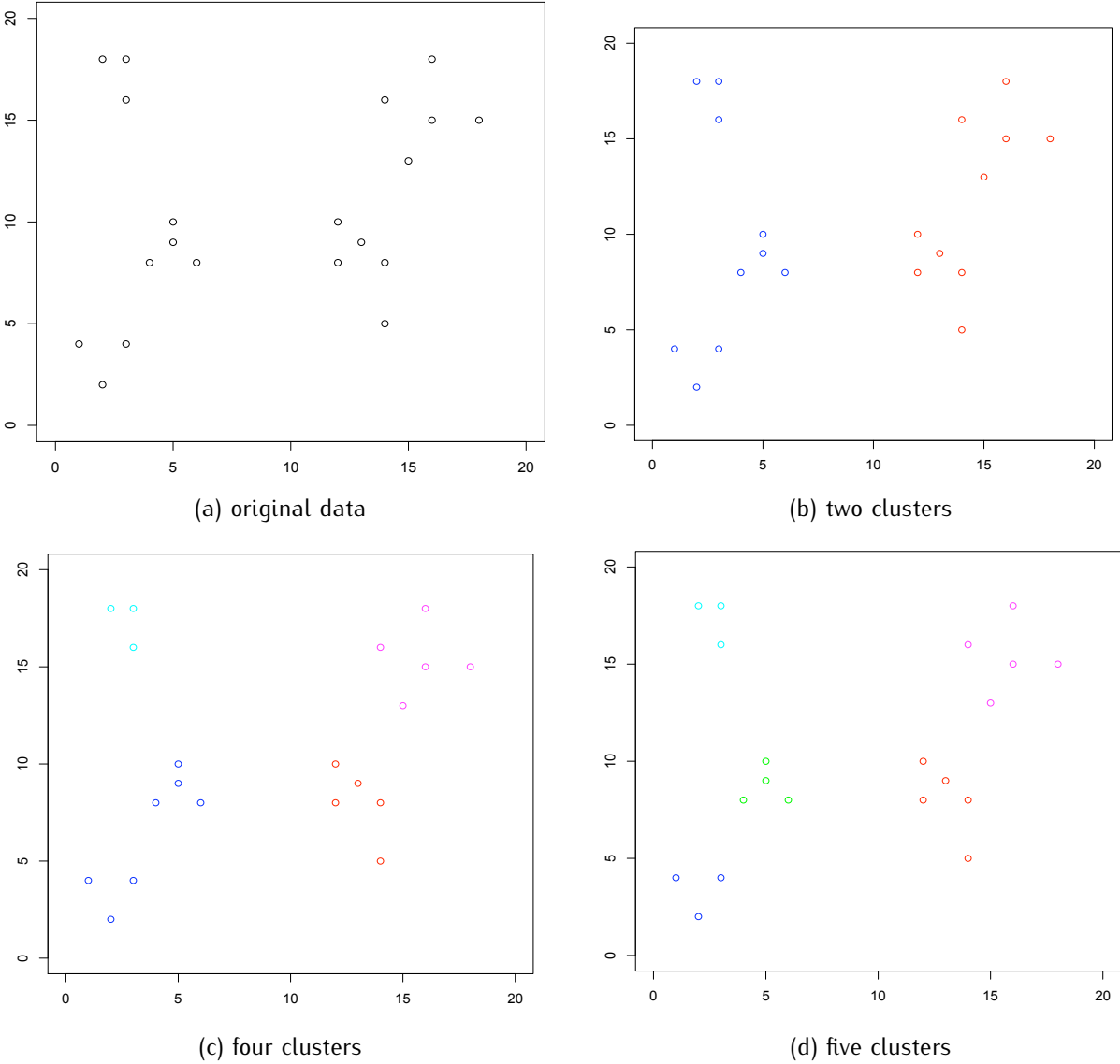
Figure 13.2: Clustering a set of 20 two-dimensional data points.
