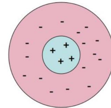
On-center, Off-surround
