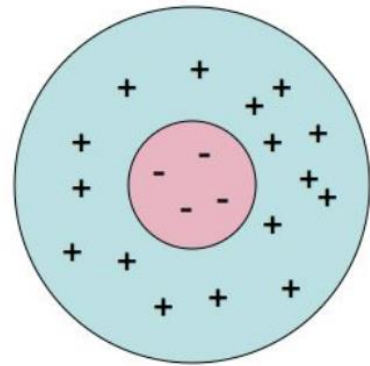
Off-center, On-surround
