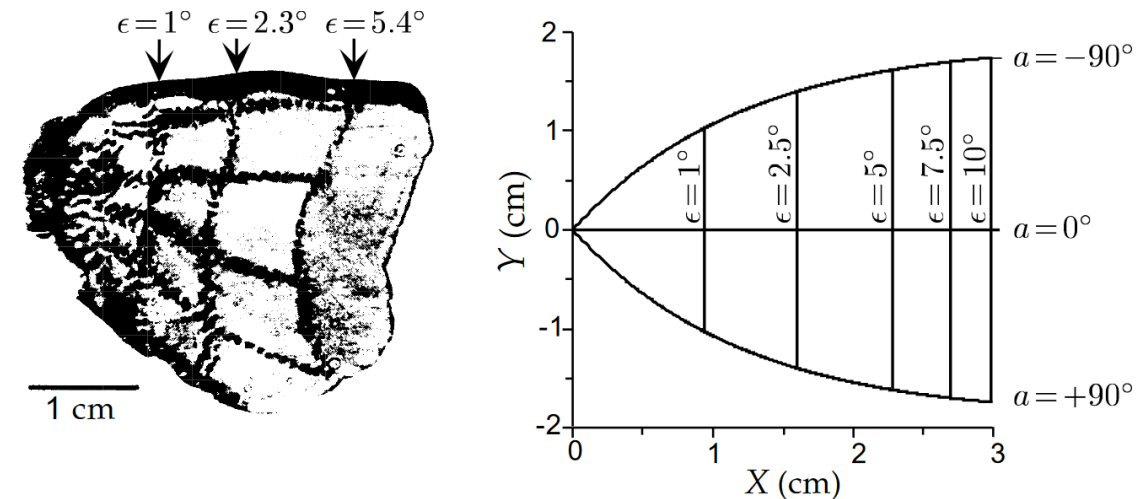
Figure 2.7 (A) An autoradiograph of the posterior region of the primary visual cortex from the left side of a macaque monkey brain. The pattern is a radioactive trace of the activity evoked by an image like that in figure 2.6B. The vertical lines correspond to circles at eccentricities of 1^\circ , 2.3^\circ , and 5.4^\circ , and the horizontal lines (from top to bottom) represent radial lines in the visual image at a values of -90^\circ , 0^\circ , 45^\circ , and 90^\circ . Only the part of cortex corresponding to the central region
