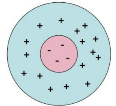
Off-center, On-surround
