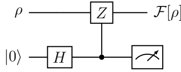
Figure 2: Channel \mathcal{F} . Hadamard gate on the ancilla followed by a controlled-Z gate.
